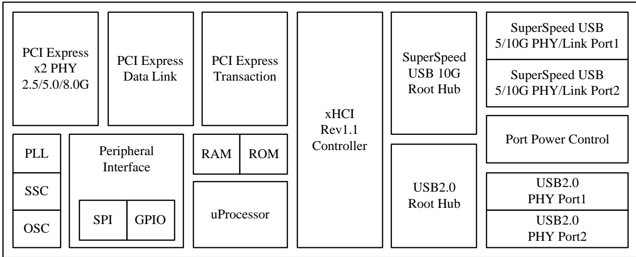
Figure 1: Functional Diagram of ASM3142
