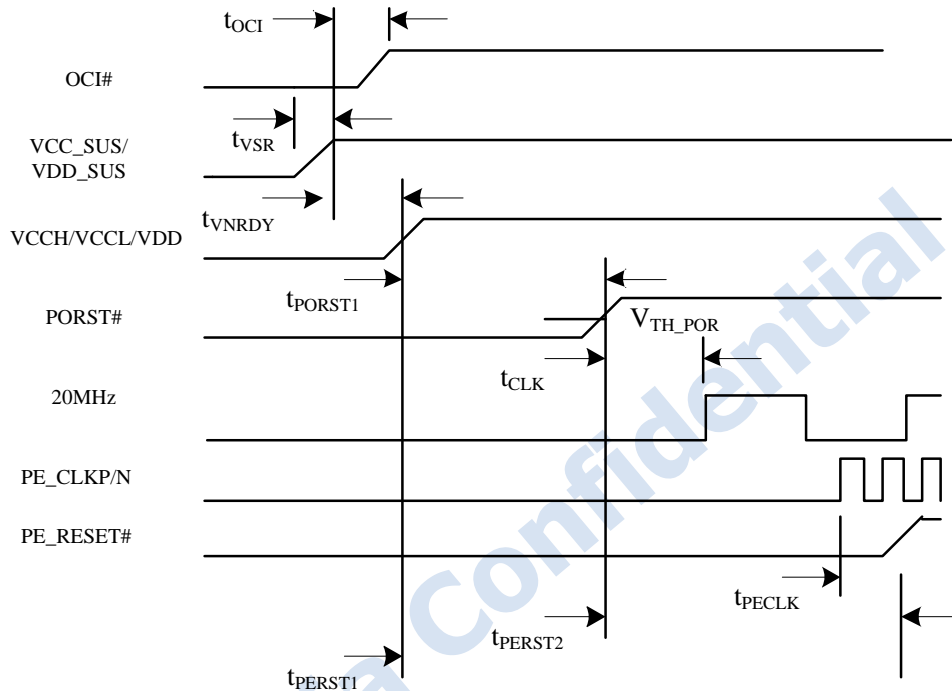
Figure 4: Power On Sequence for Asynchronous mode
