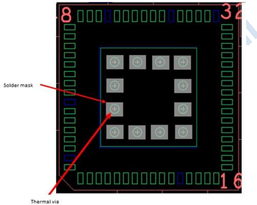
Figure 6: Symbol 1 for via design rule under Thermal pad
