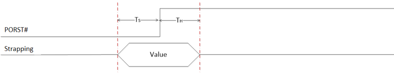
Figure 5: timing for strapping
